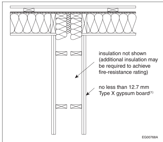
Figure A-9.36.2.5.(2)-C Penetrating element insulated within itself
