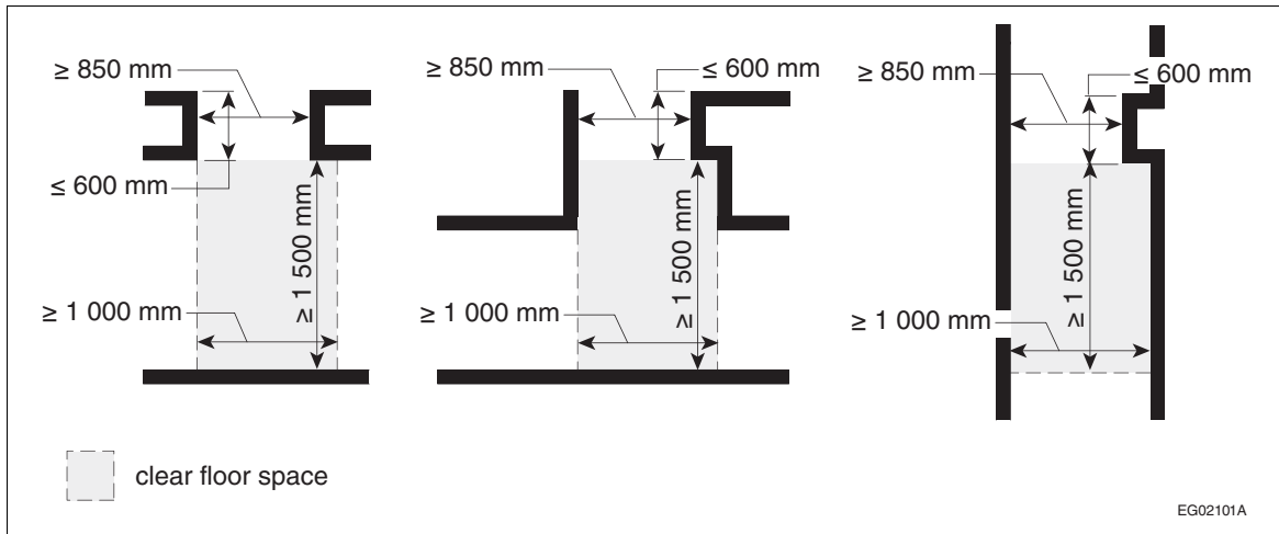
Figure A-3.8.3.2(2) Barrier-free paths of travel with a reduced clear-width section
