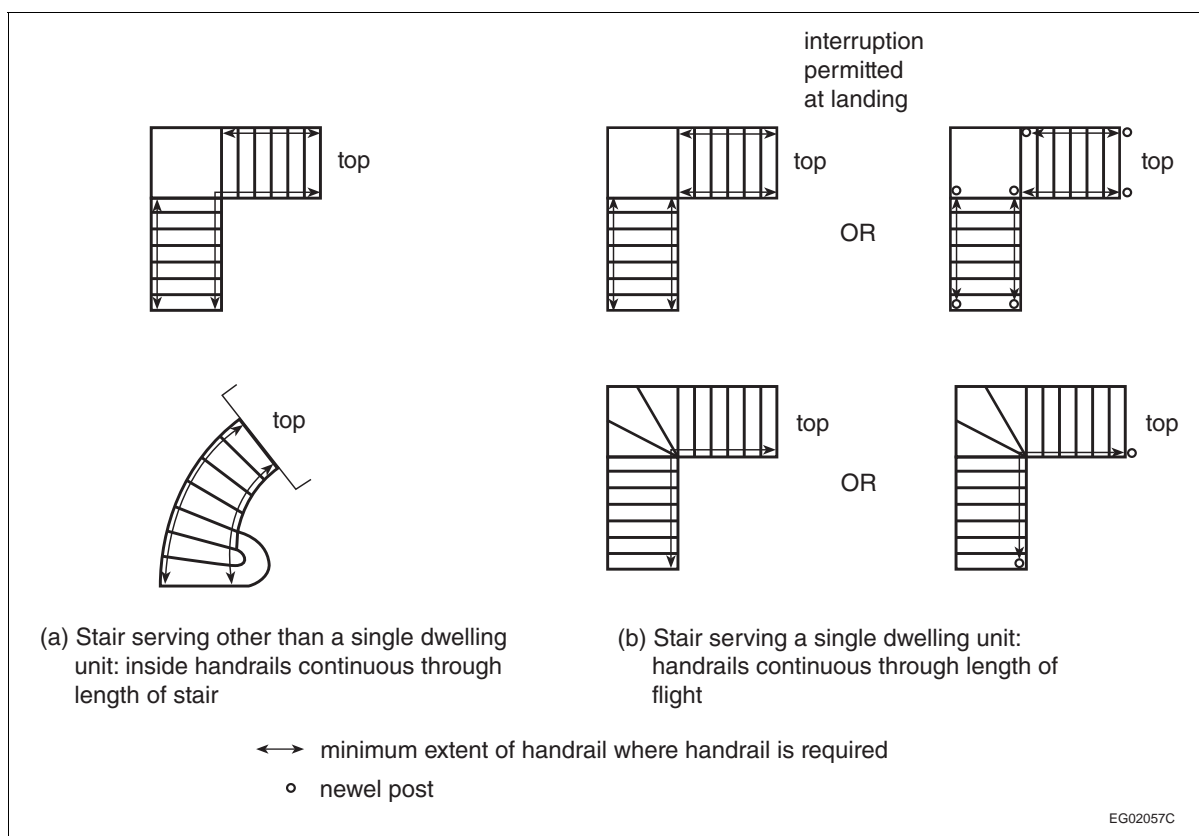
Figure A-9.8.7.2. Continuity of handrails at the top and bottom of stairs and flights
