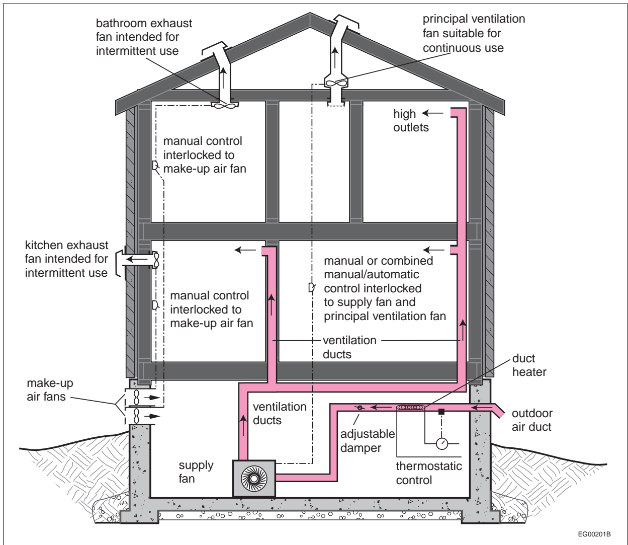
Figure A-9.32.3.3-C
