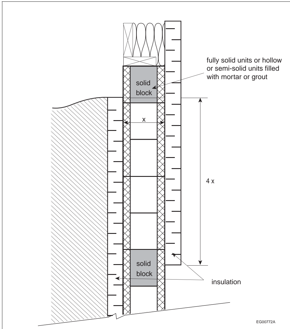
Figure A-9.36.2.5.(5)-B
