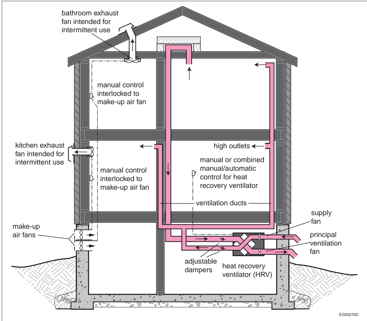
Figure A-9.32.3.3.-D
